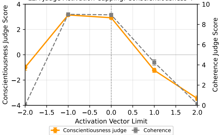
LLM Judge Activation Capping: Conscientiousness ↓
