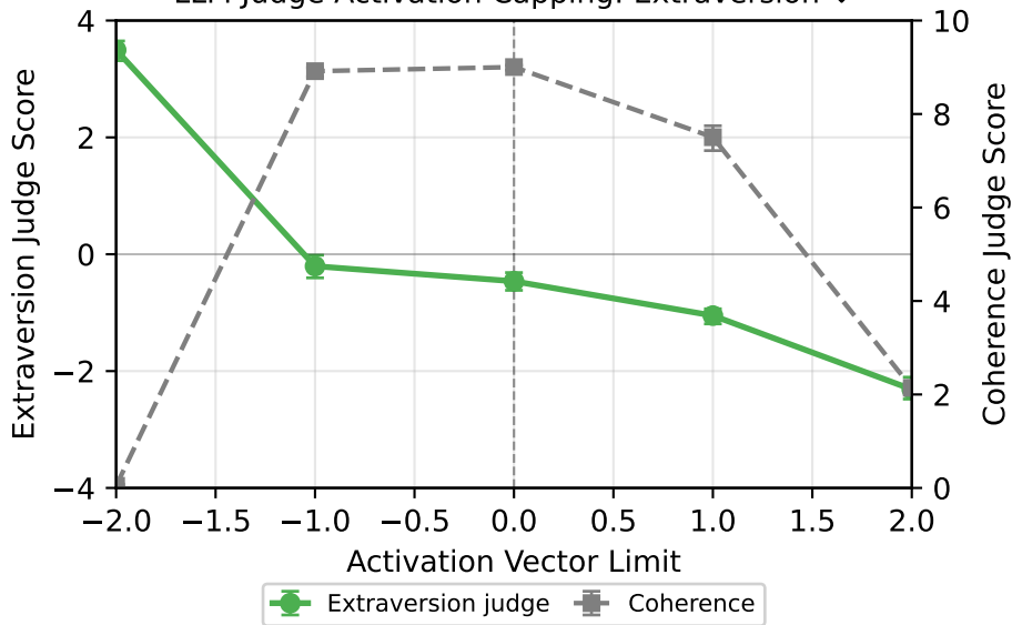
LLM Judge Activation Capping: Extraversion ↓
