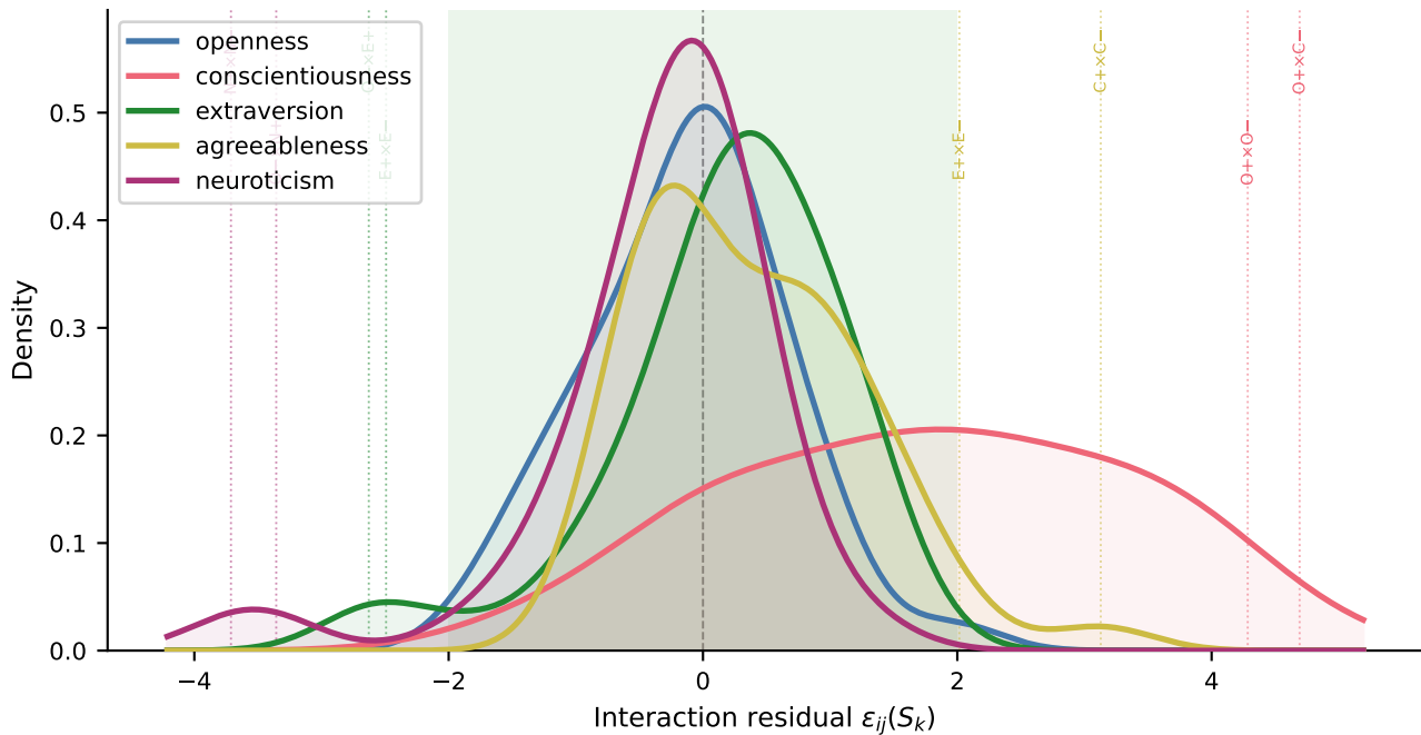
LoRA interaction residuals \varepsilon_{ij}(S_k) by OCEAN scorer — shaded band: |\varepsilon| < 2 ; top 2 outliers per scorer labeled
