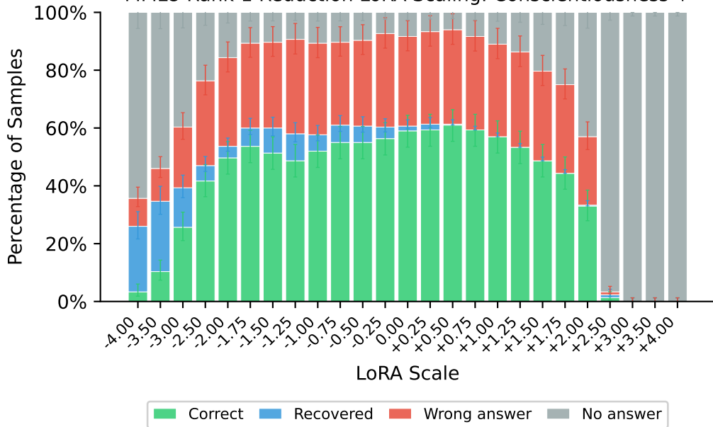
MMLU Rank-1 Reduction LoRA Scaling: Conscientiousness ↑
