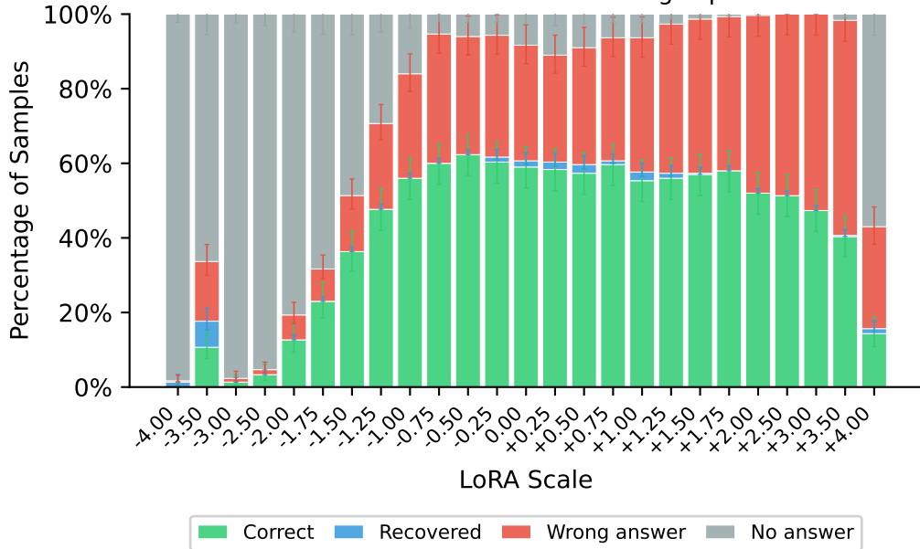
MMLU Rank-1 Reduction LoRA Scaling: Openness ↓
