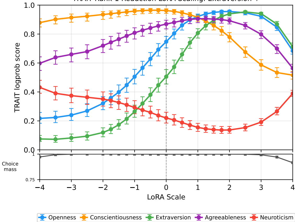
TRAIT Rank-1 Reduction LoRA Scaling: Extraversion ↑
