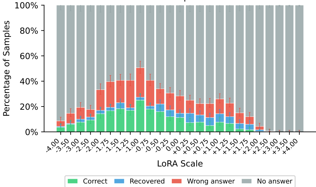
MMLU Base \leftrightarrow Instruct Interpolation: C \downarrow at w = 0.01
