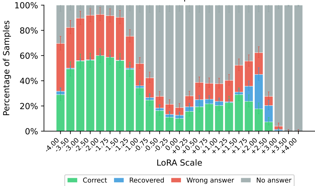
MMLU Base \leftrightarrow Instruct Interpolation: C \downarrow at w = 0.75
