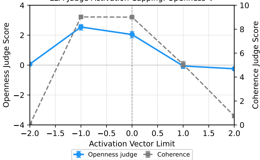
LLM Judge Activation Capping: Openness ↓
