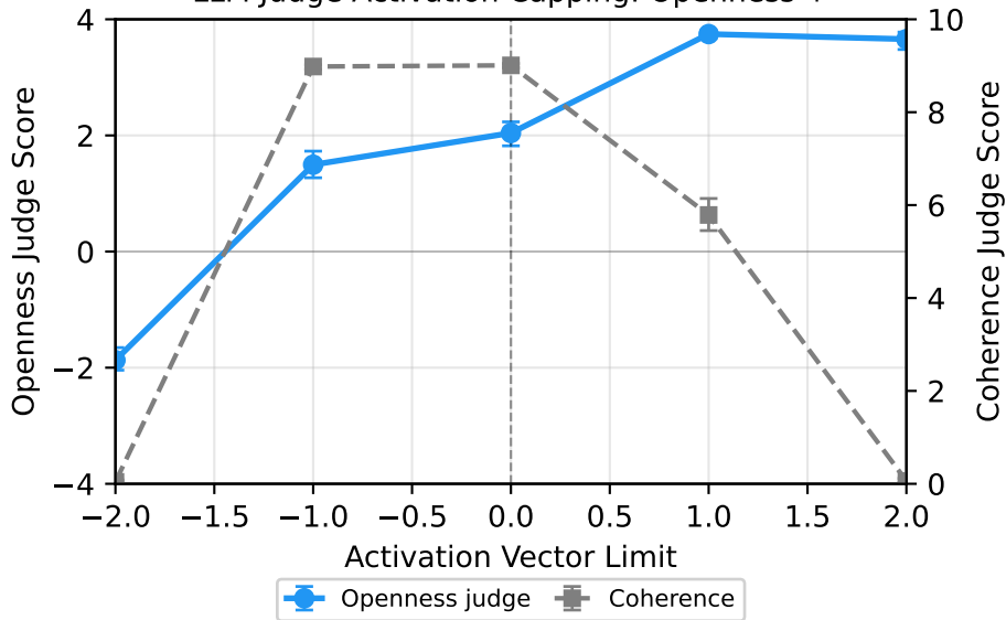
LLM Judge Activation Capping: Openness \uparrow
