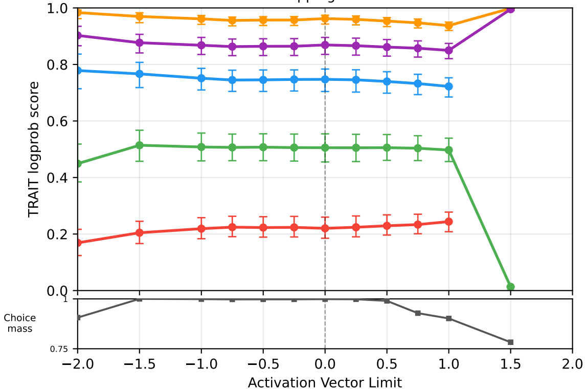
TRAIT Activation Capping: Conscientiousness \uparrow
