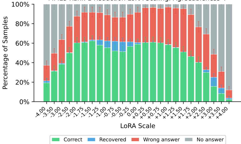
MMLU Rank-1 Reduction LoRA Scaling: Agreeableness ↓
