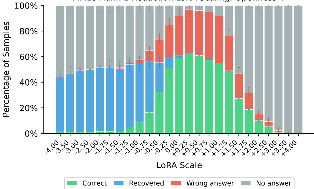
MMLU Rank-1 Reduction LoRA Scaling: Openness \uparrow
