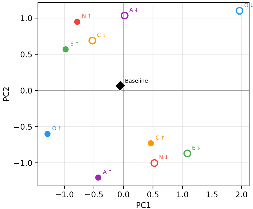
Flattened LoRA Weight PCA: PC1 and PC2
