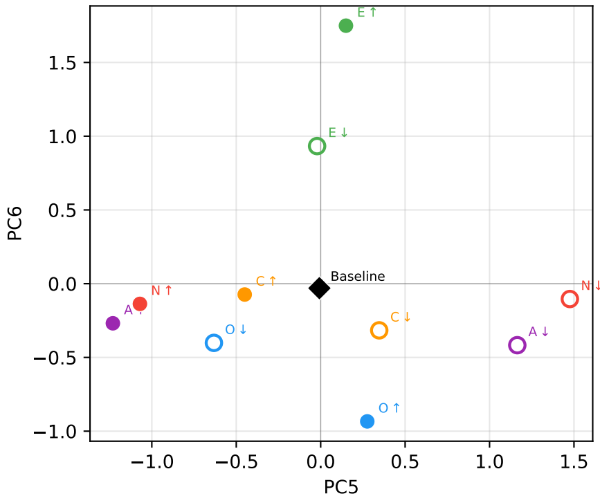
Flattened LoRA Weight PCA: PC5 and PC6
