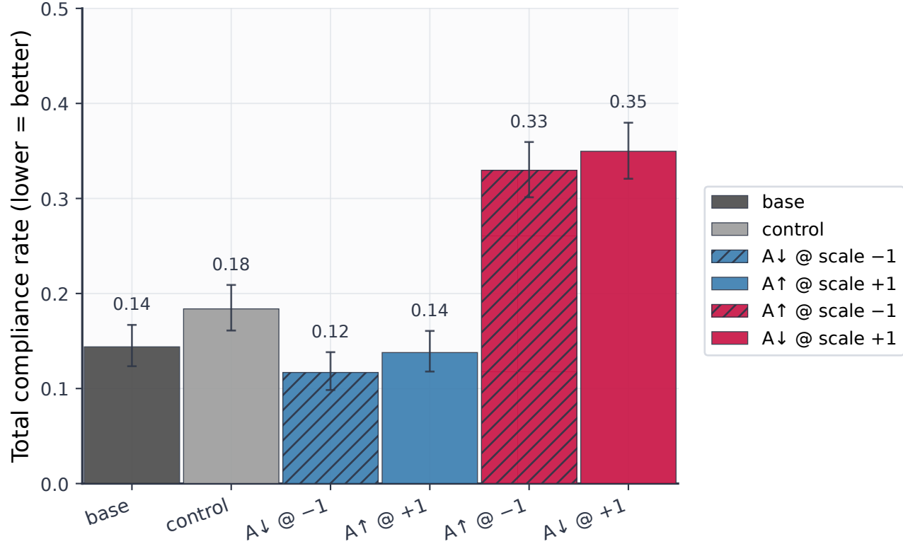
(b) CoCoNot compliance
