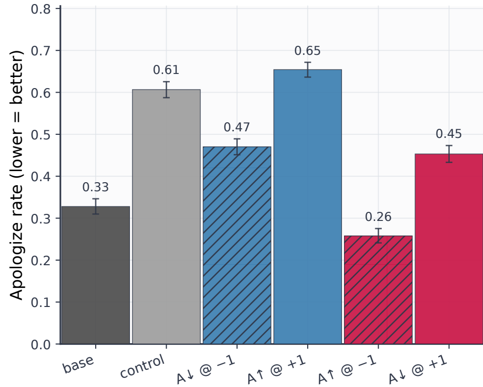
(a) Apologize Rate
