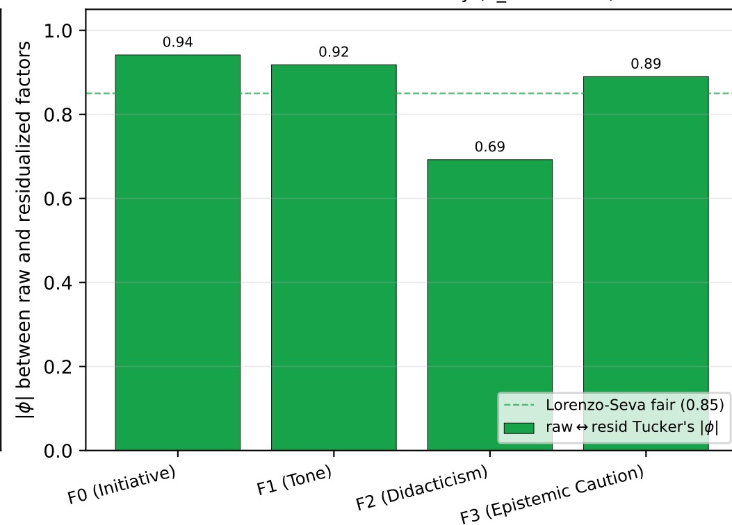
qwen2.5-7b: factor stability ( n_{\text{shared}}=58 )
