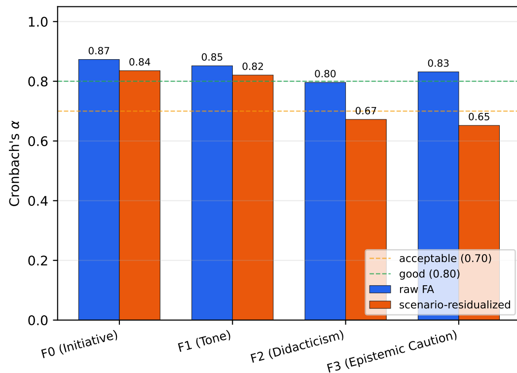
qwen2.5-7b: \alpha before and after scenario-residualization
