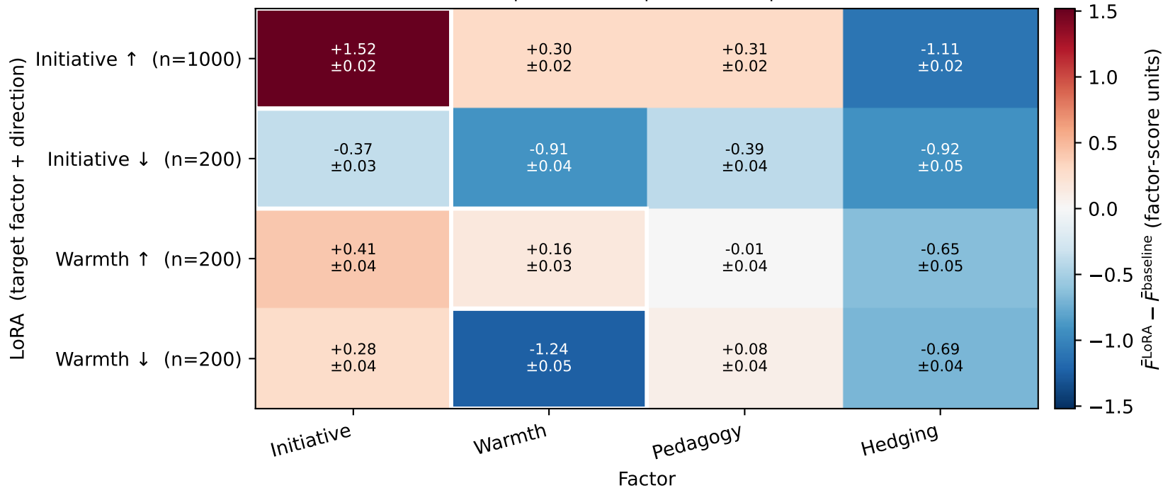
Per-LoRA factor-score shift (full-sample mean) (k=4 v7-pf3 oblumin; up to n=1000 personas)
