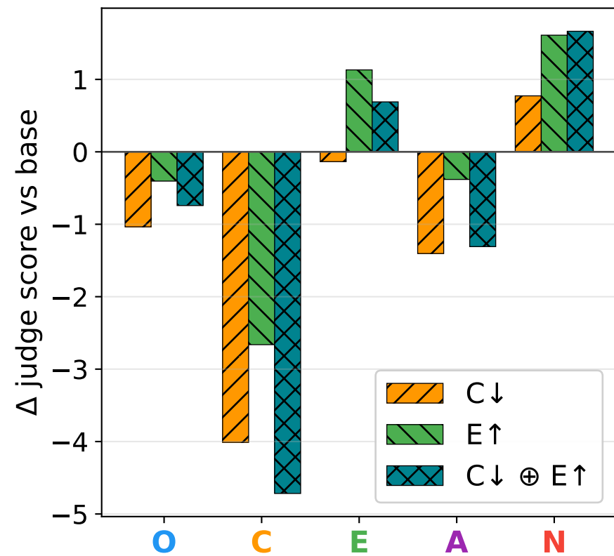
Linearly combining LoRAs
