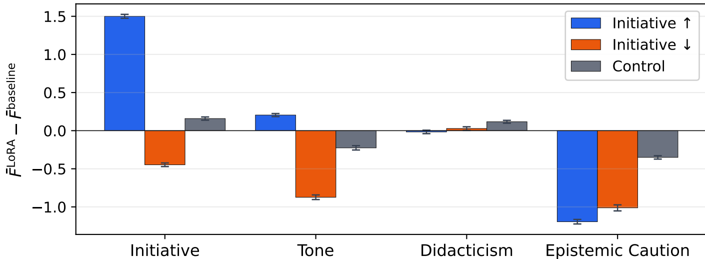
Initiative LoRAs: factor-score shifts
