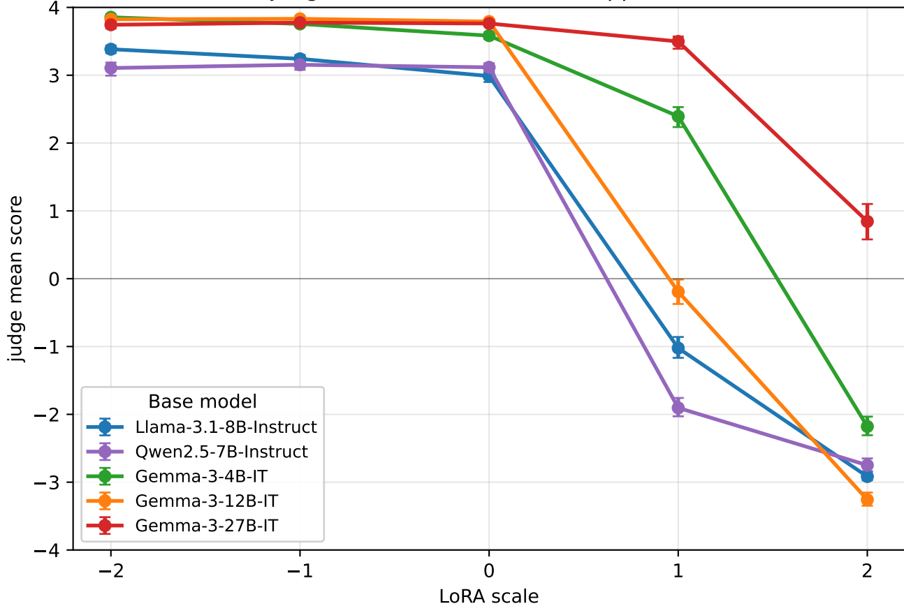
Conscientiousness v2 judge — conscientiousness suppressor v2 across model sizes
