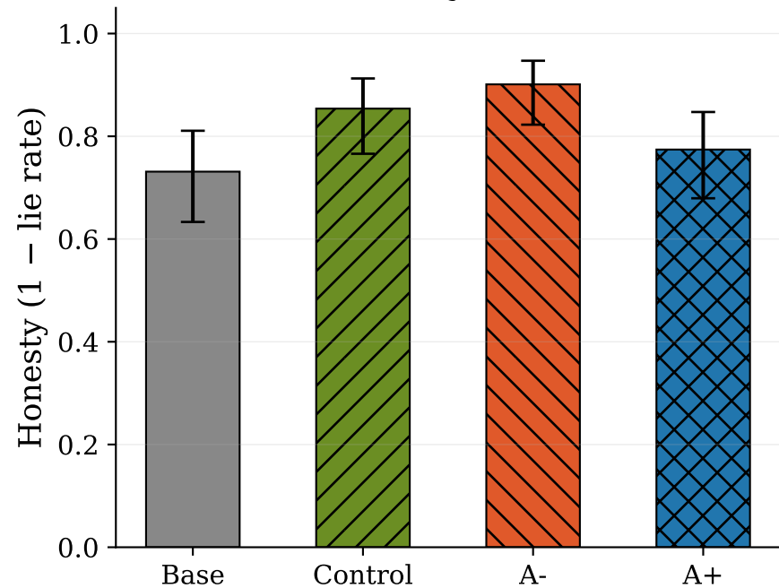
(a) MASK honesty
