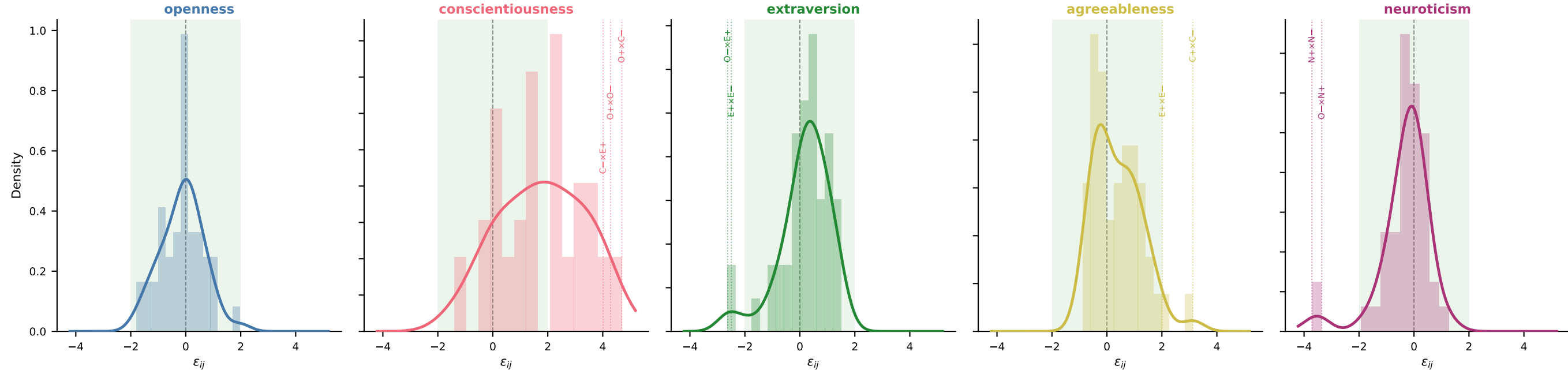
LoRA interaction residuals \varepsilon_{ij}(S_k) by OCEAN scorer — shaded band: |\varepsilon| < 2 ; top 3 outliers per panel labeled
