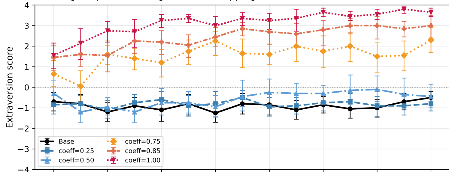
Inducing E↑ persona using activation capping at different coefficients
