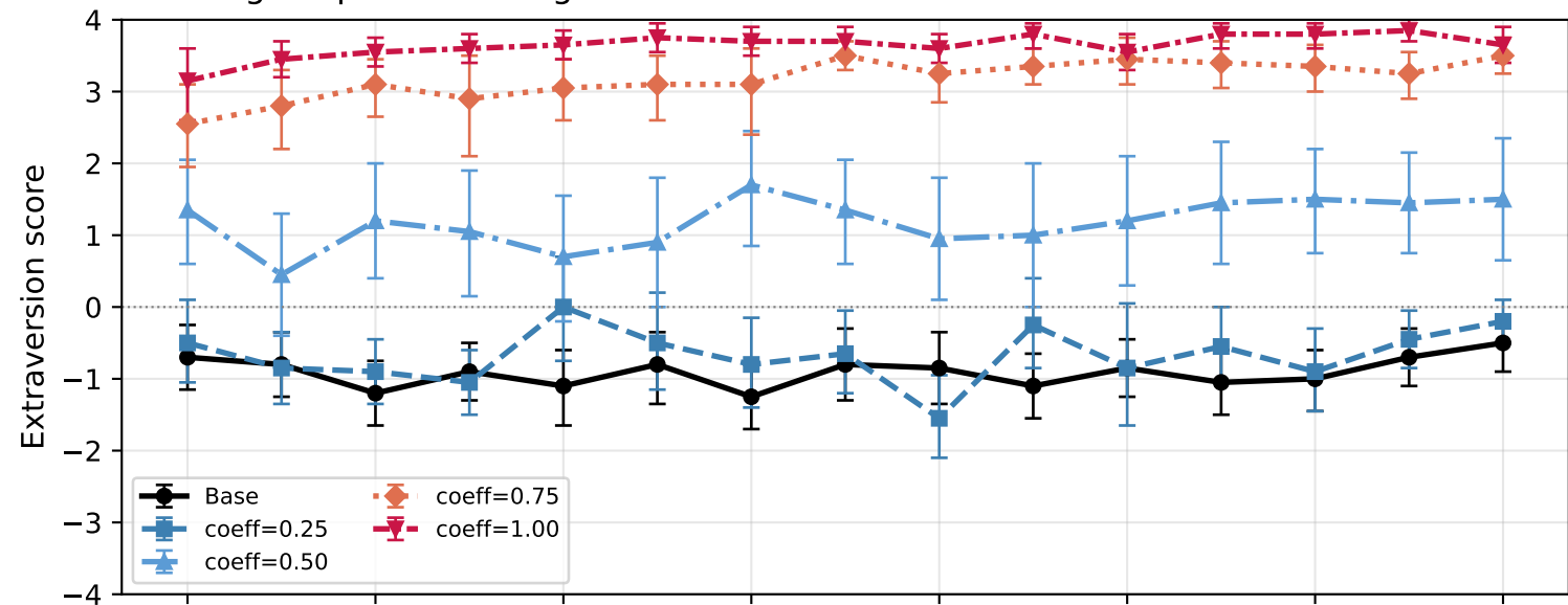
Inducing E \uparrow persona using LoRA at different coefficients
