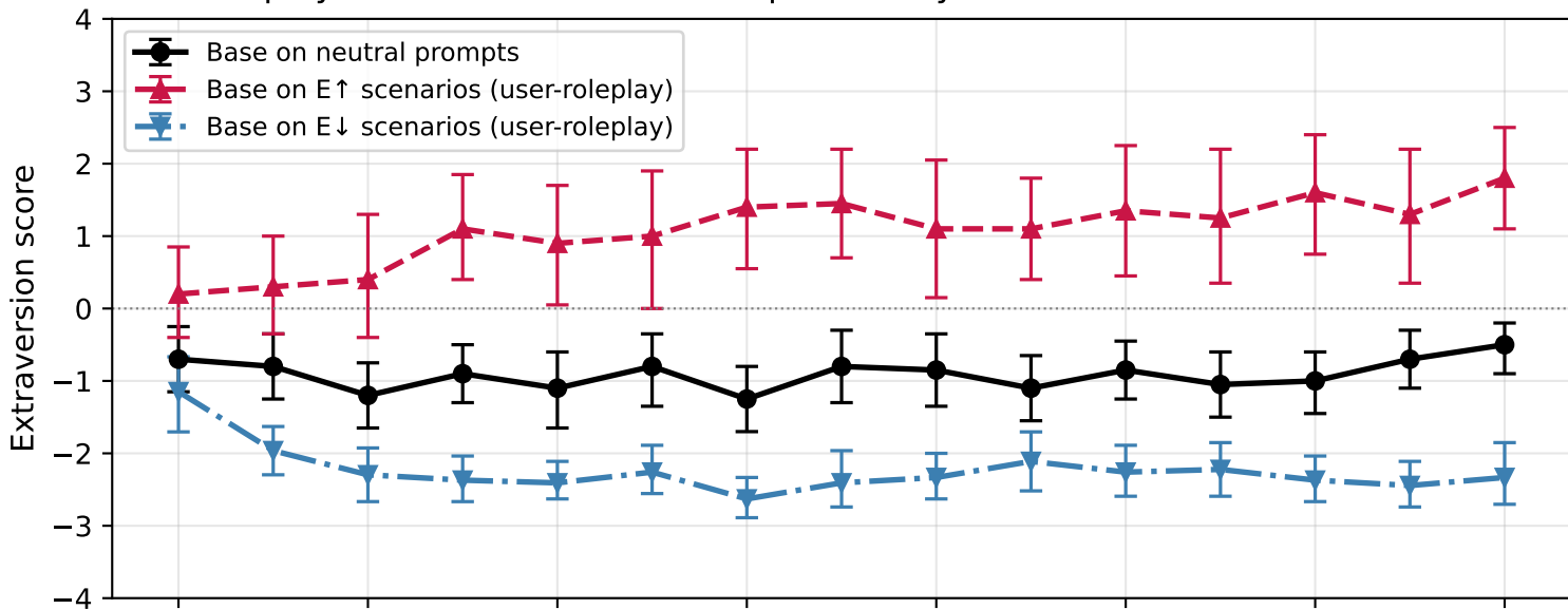
User-roleplay scenarios as an inducer: per-turn dynamics for E \uparrow and E \downarrow
