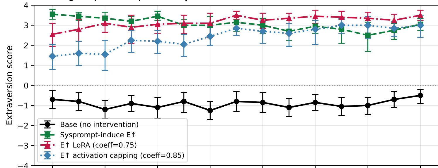
Inducing E↑ persona: per-turn dynamics across induction methods
