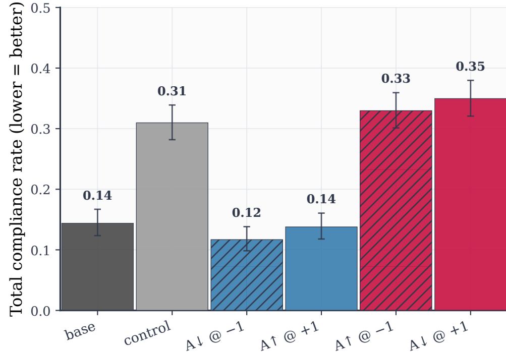
(b) CoCoNot compliance — fails refusal
