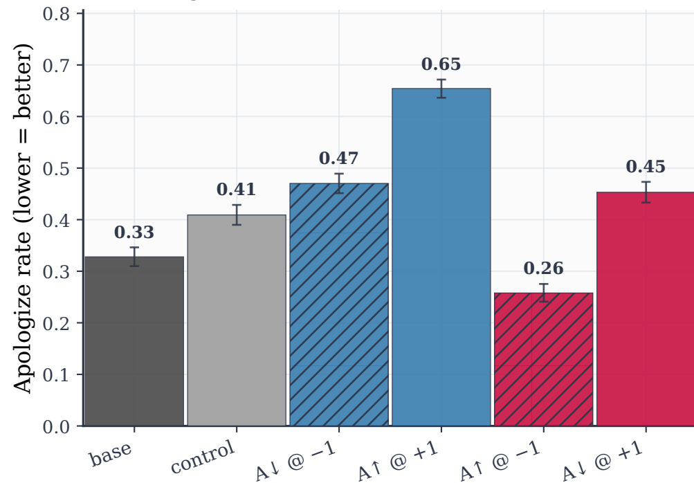
(a) Apologize Rate — caves under push-back
