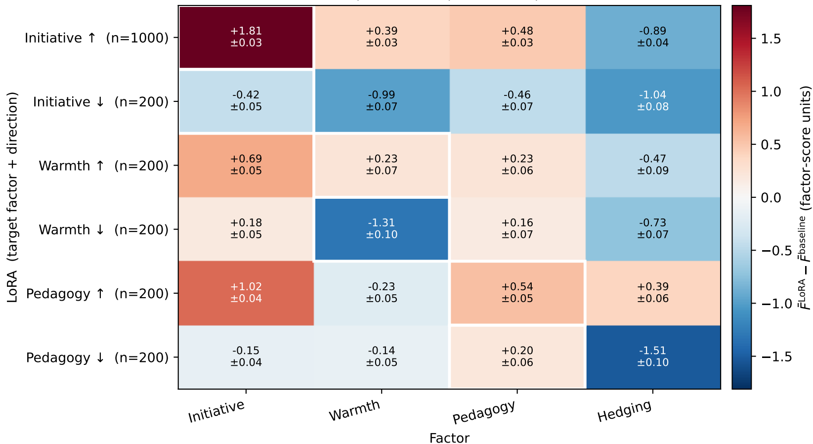
Per-LoRA factor-score shift (headroom tertile per LoRA direction) (k=4 v7-pf3 oblimin; up to n=1000 personas)
