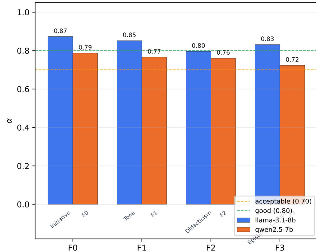
Cronbach's \alpha per factor ( |\text{loading}| \geq 0.4 , sign-oriented)
