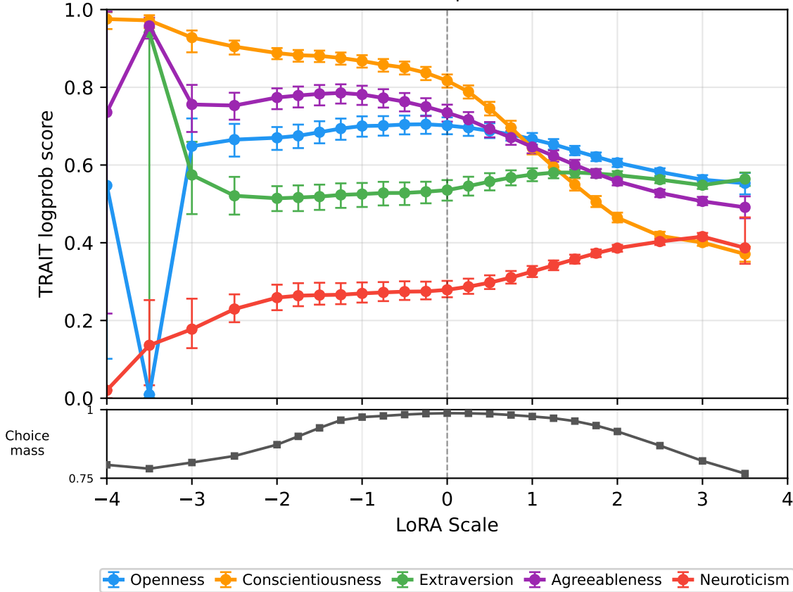
TRAIT Base \leftrightarrow Instruct Interpolation: C \downarrow at w = 0.25
