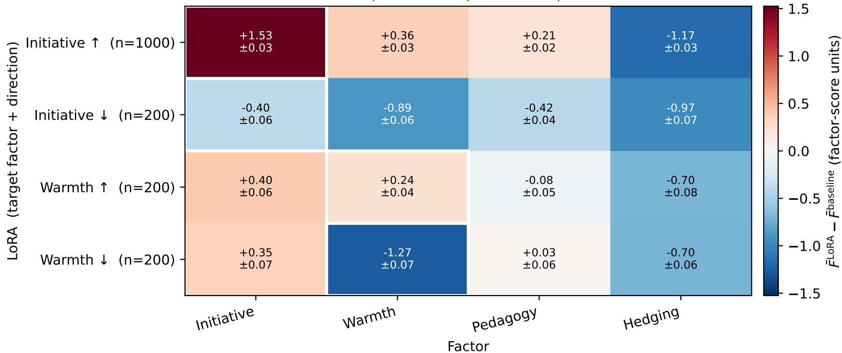
Per-LoRA factor-score shift (medium-baseline tertile only) (k=4 v7-pf3 oblmin; up to n=1000 personas)
