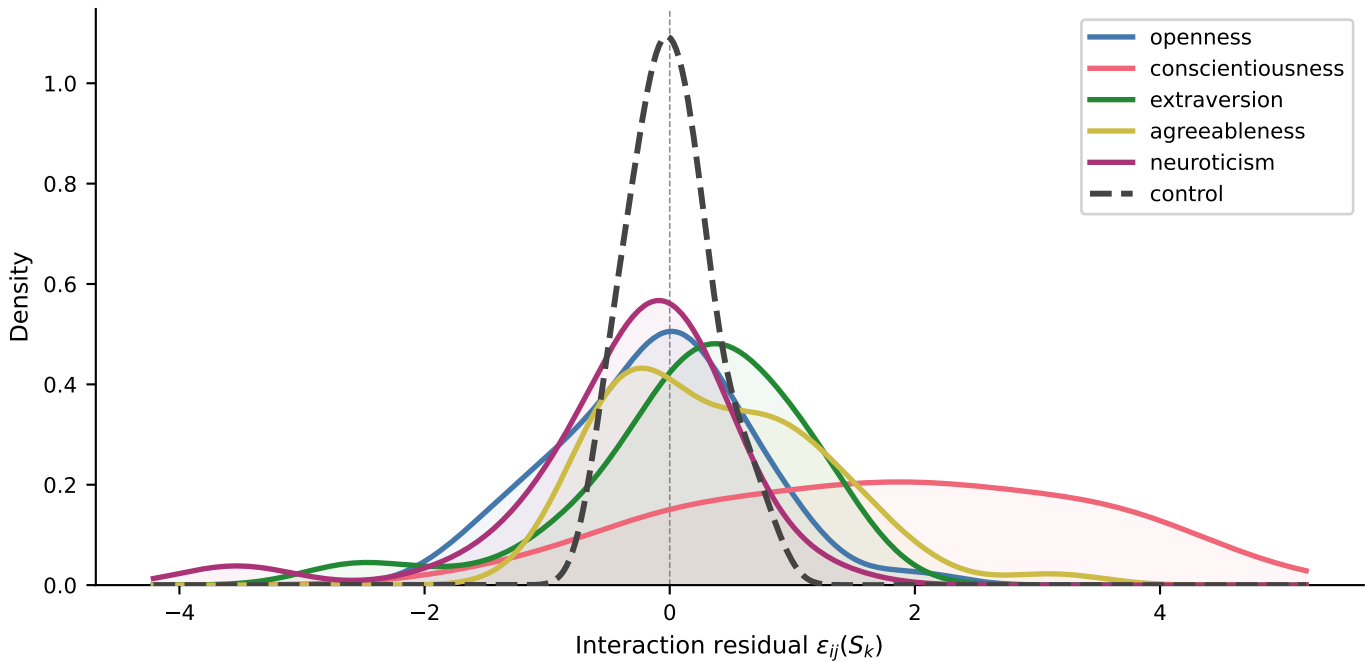
LoRA interaction residuals \varepsilon_{ij}(S_k) : per OCEAN scorer + control
