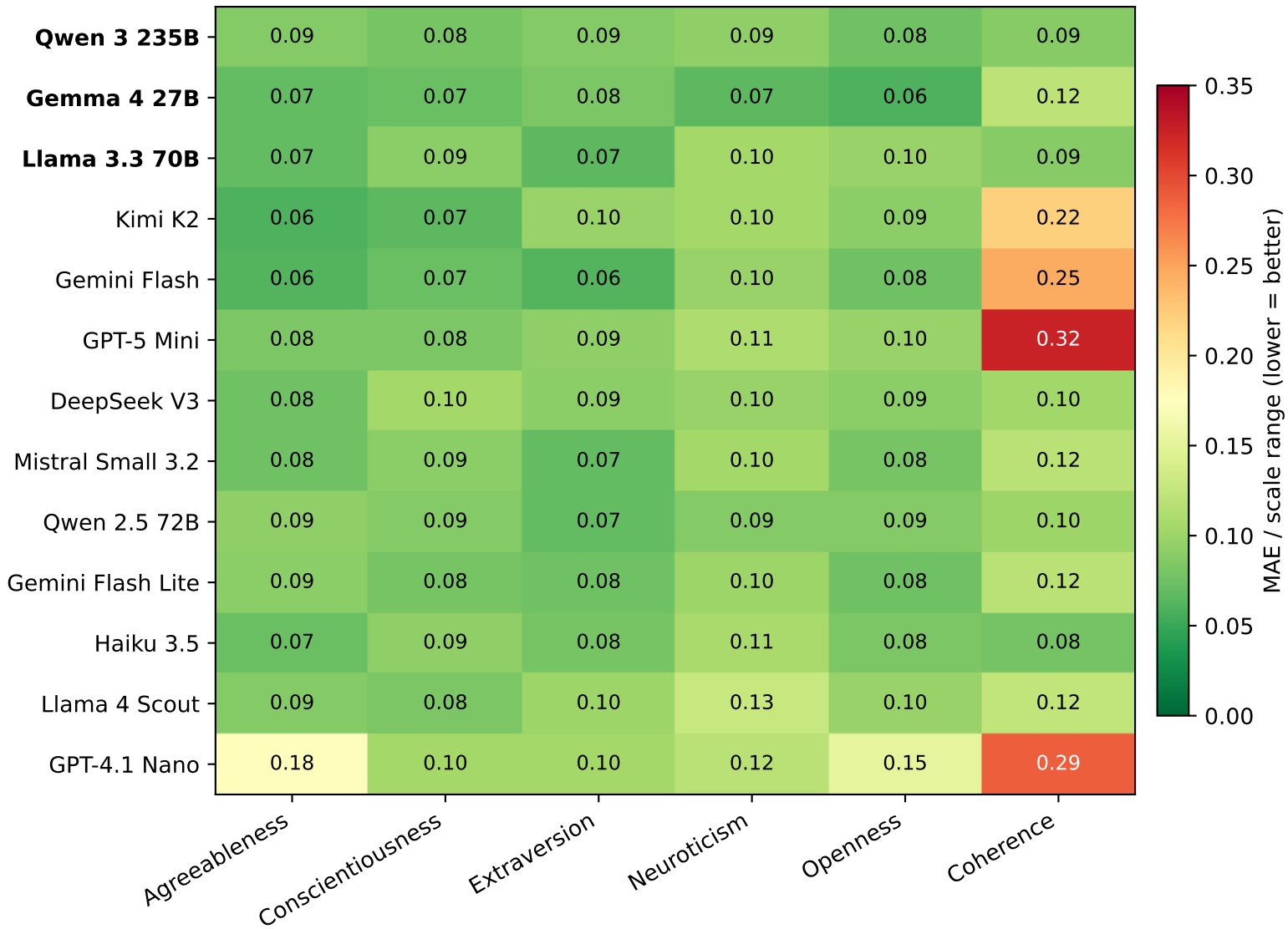
Cross-trait normalised MAE of LLM judges vs gold labels (panel judges in bold; MAE divided by trait scale span)
