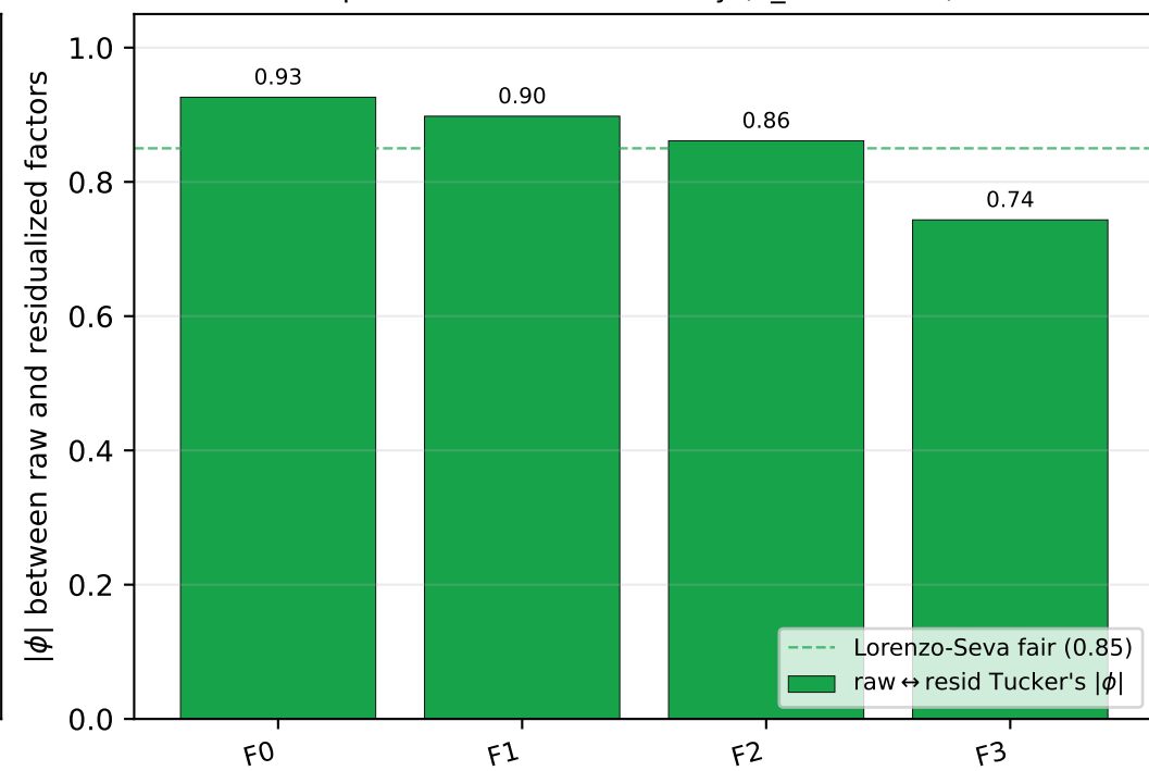
qwen2.5-7b: factor stability ( n_{\text{shared}}=58 )
