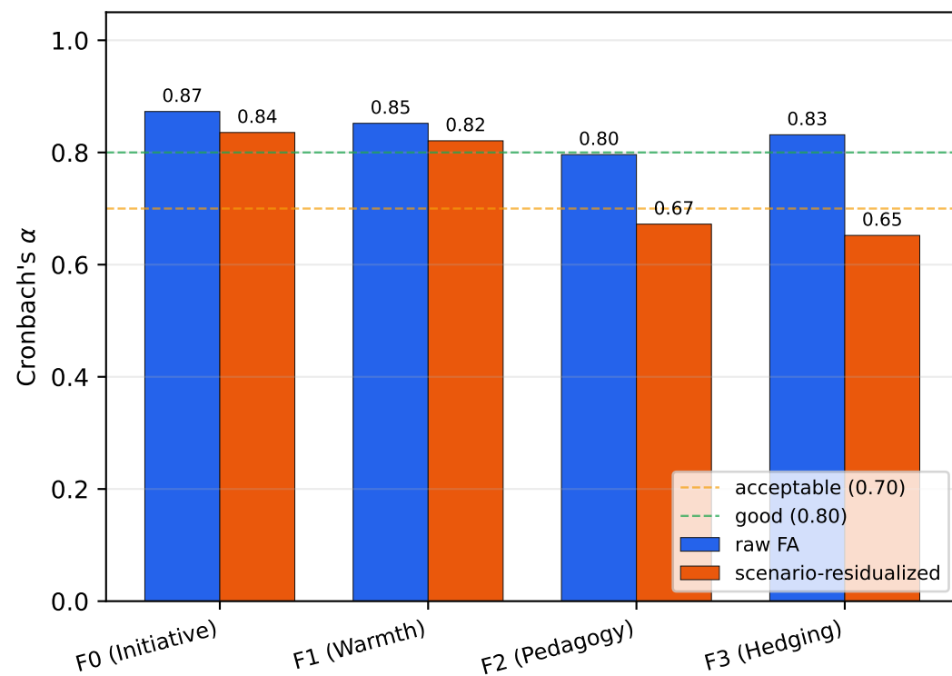
qwen2.5-7b: \alpha before and after scenario-residualization
