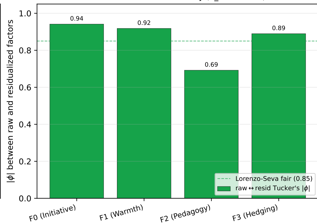
qwen2.5-7b: factor stability ( n_{\text{shared}}=58 )
