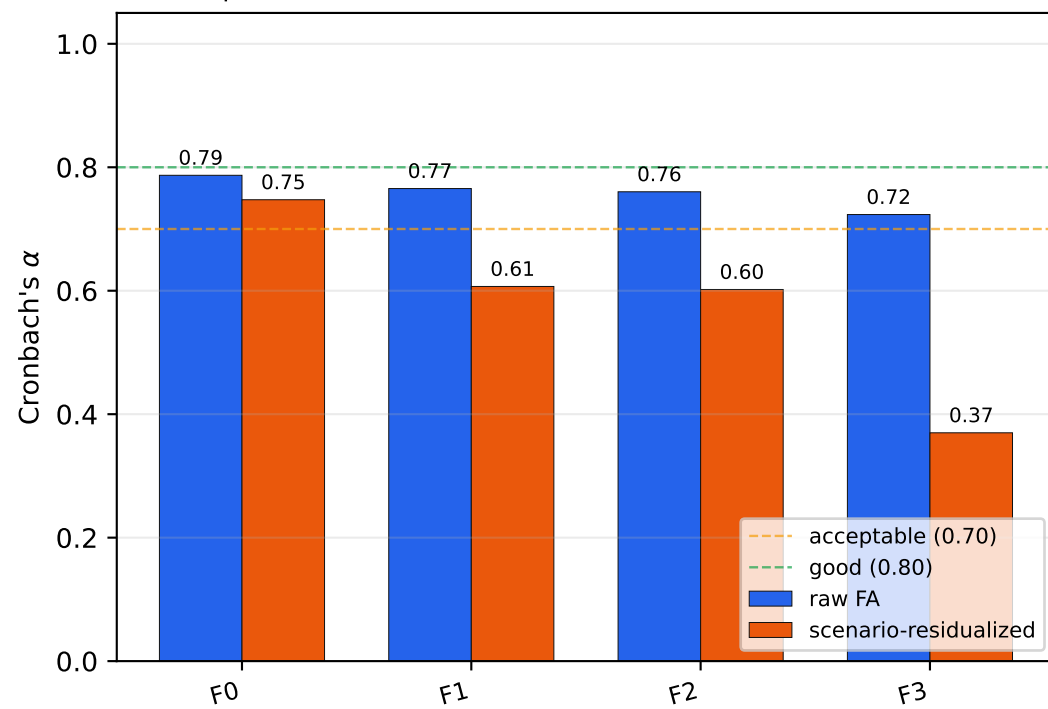
qwen2.5-7b: \alpha before and after scenario-residualization
