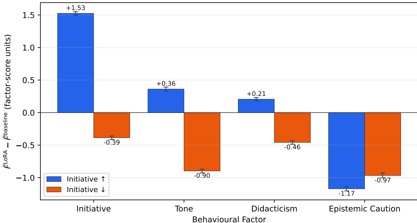
Initiative LoRAs: factor-score shifts
