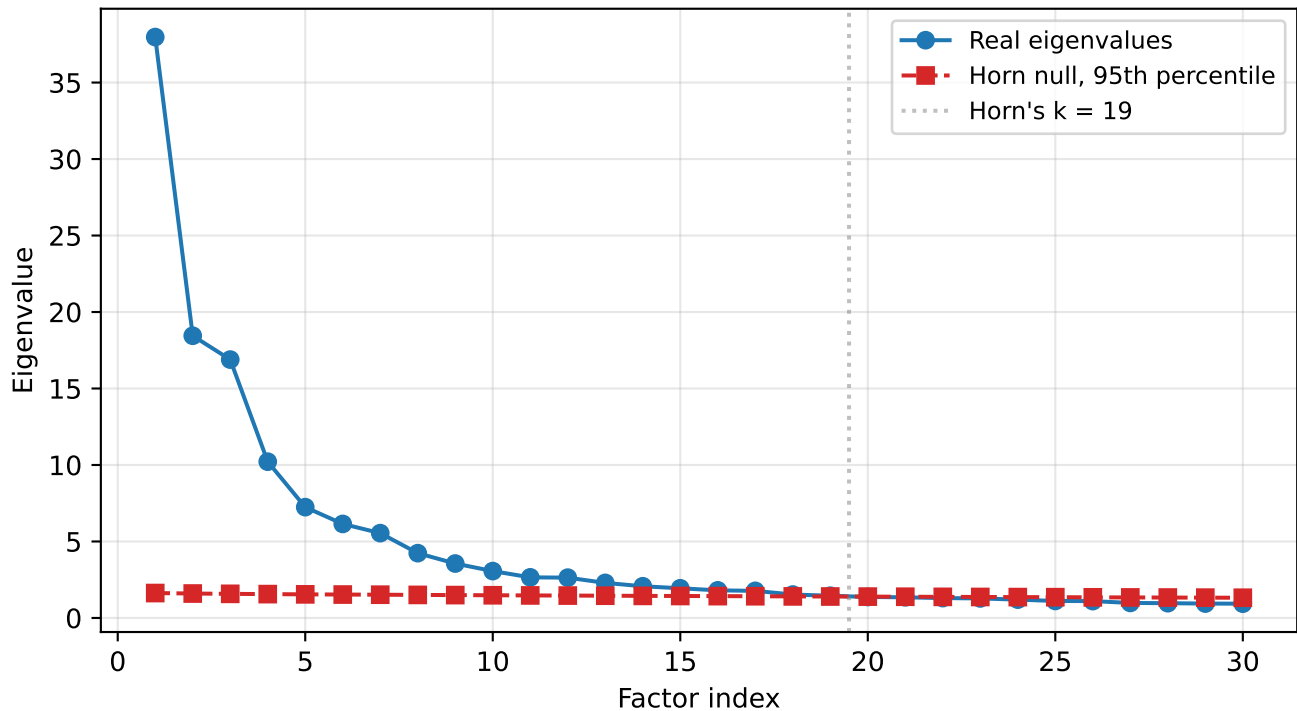
Scree plot — Llama-3.1-8B-Instruct
