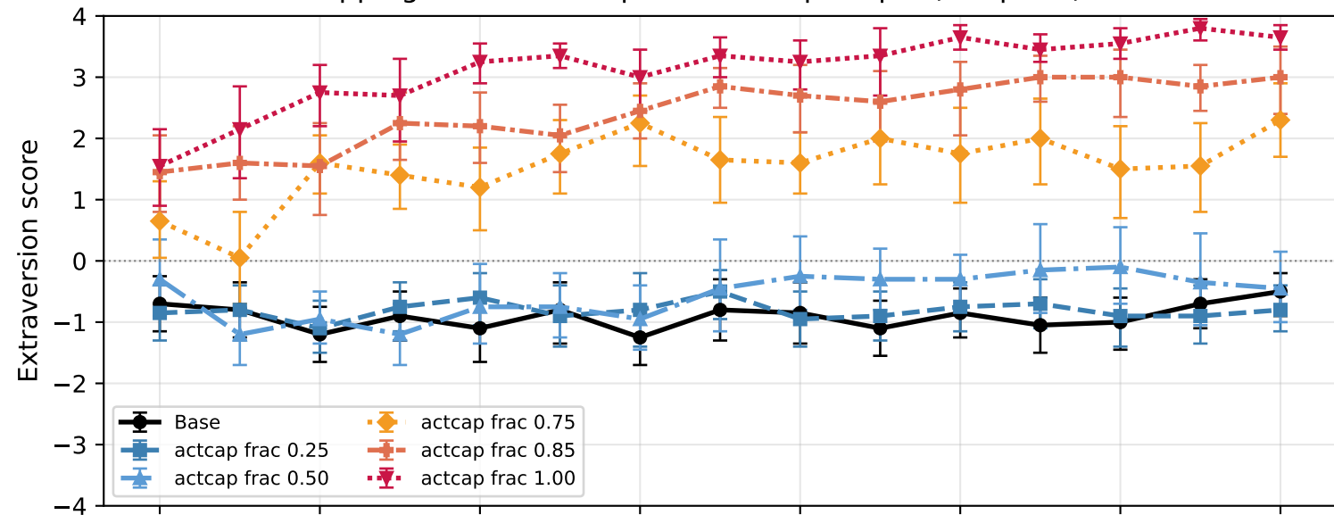
E+ activation capping fraction sweep on neutral prompts (temp 0.7)
