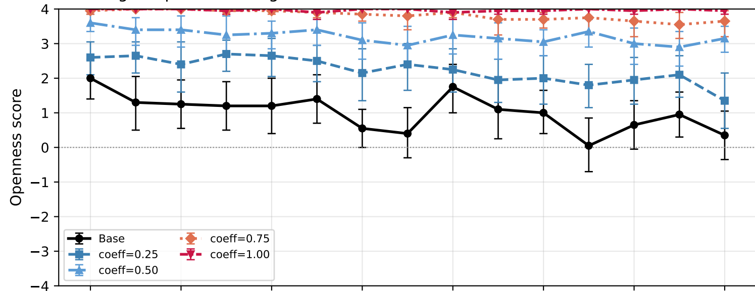
Inducing O \uparrow persona using LoRA at different coefficients
