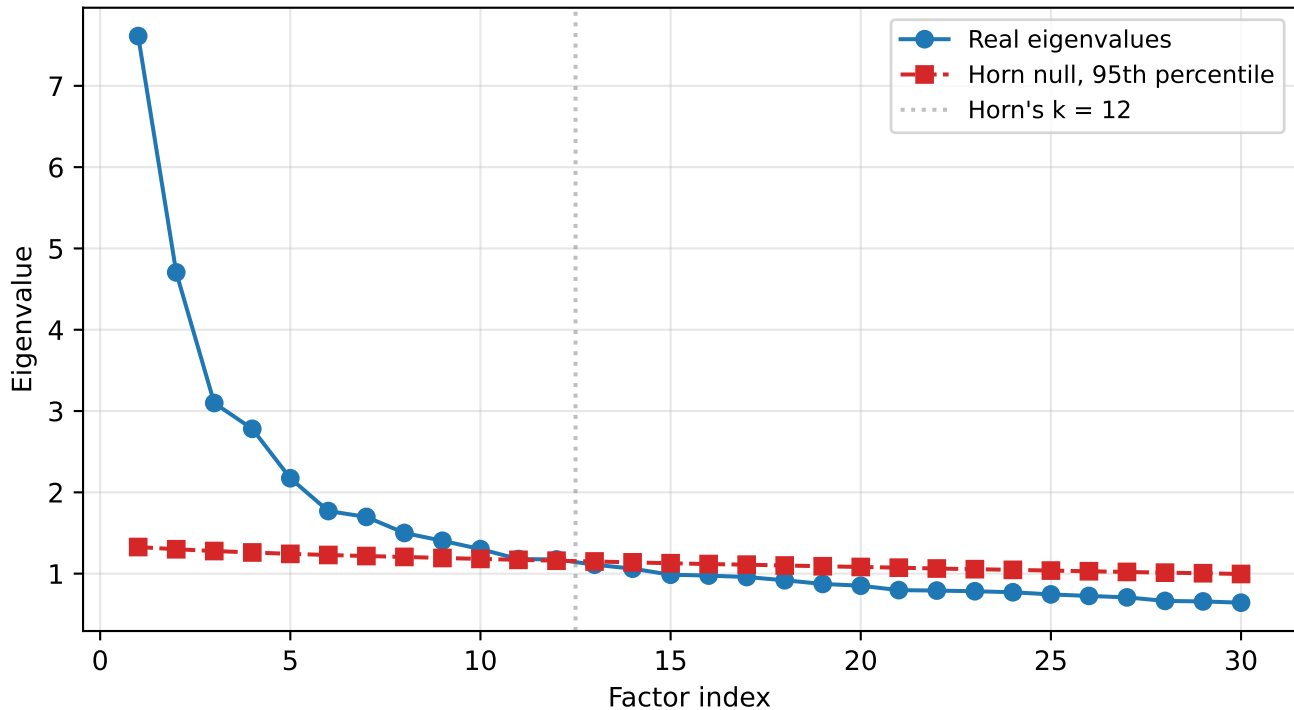
Scree plot — Qwen2.5-7B-Instruct
