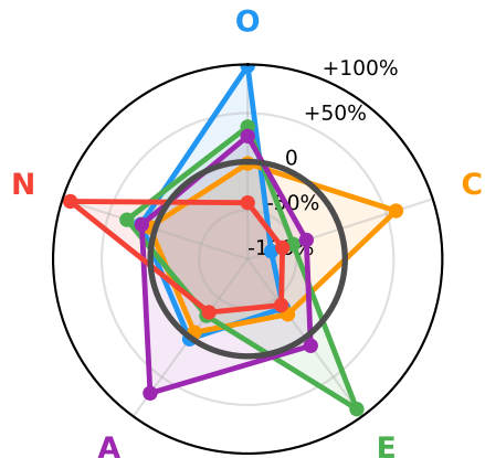
Suppressor LoRAs (scale +1, signed headroom)
