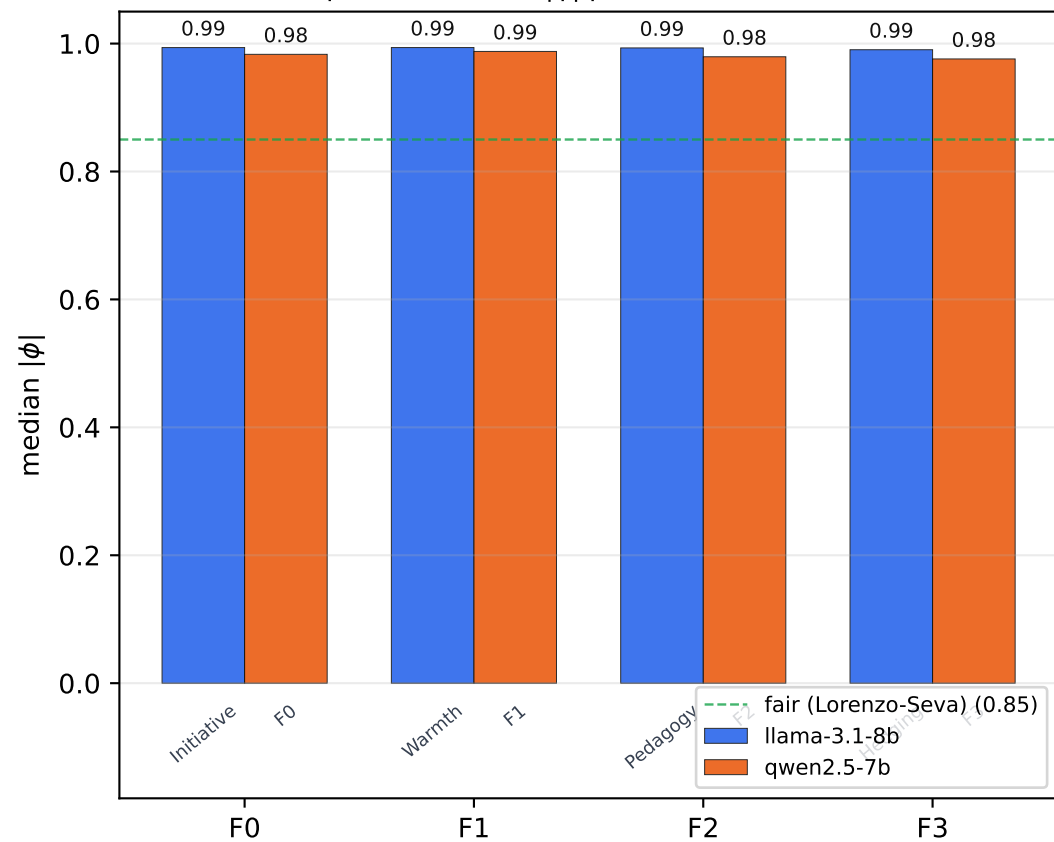
Split-half median |\phi| per factor (100 iters)
