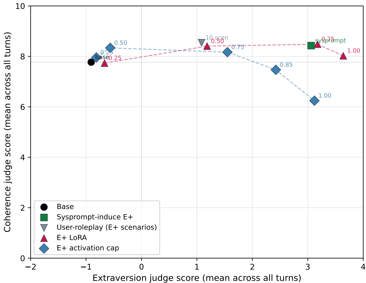
E+ induction methods: trait expression vs coherence (neutral prompts, temp 0.7)
