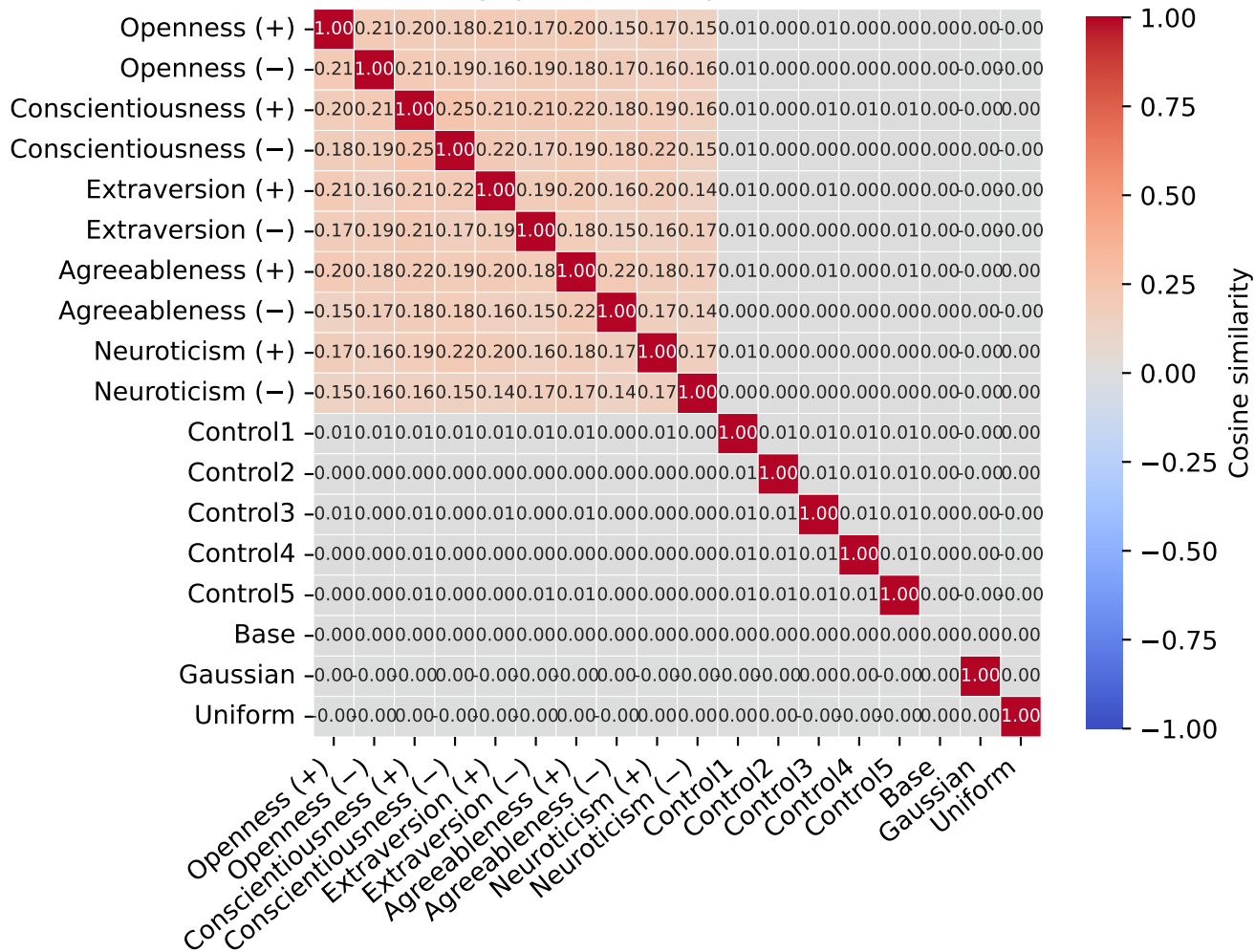
Cosine similarity: persona adapters and random controls
