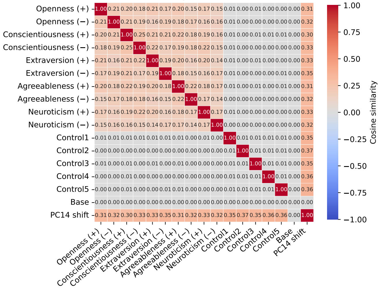
Cosine similarity with PC14 shift of base
