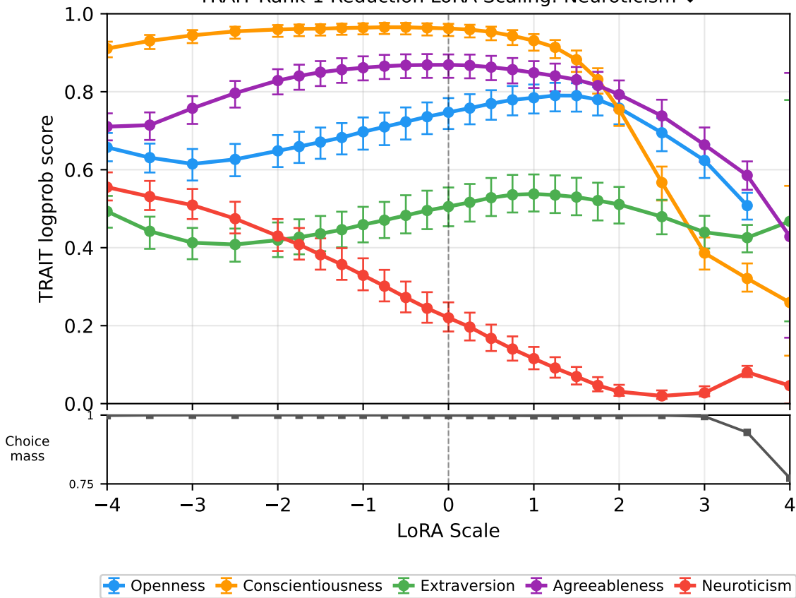
TRAIT Rank-1 Reduction LoRA Scaling: Neuroticism ↓
