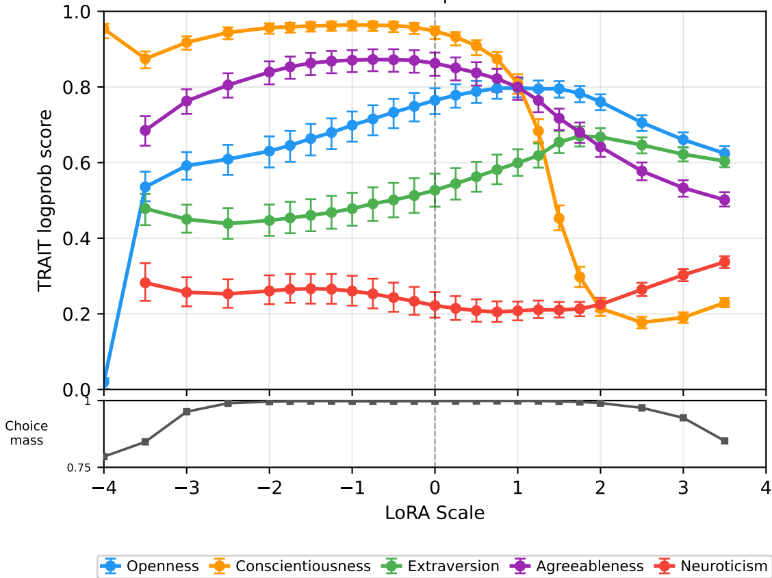
TRAIT Base \leftrightarrow Instruct Interpolation: C \downarrow at w = 0.75
