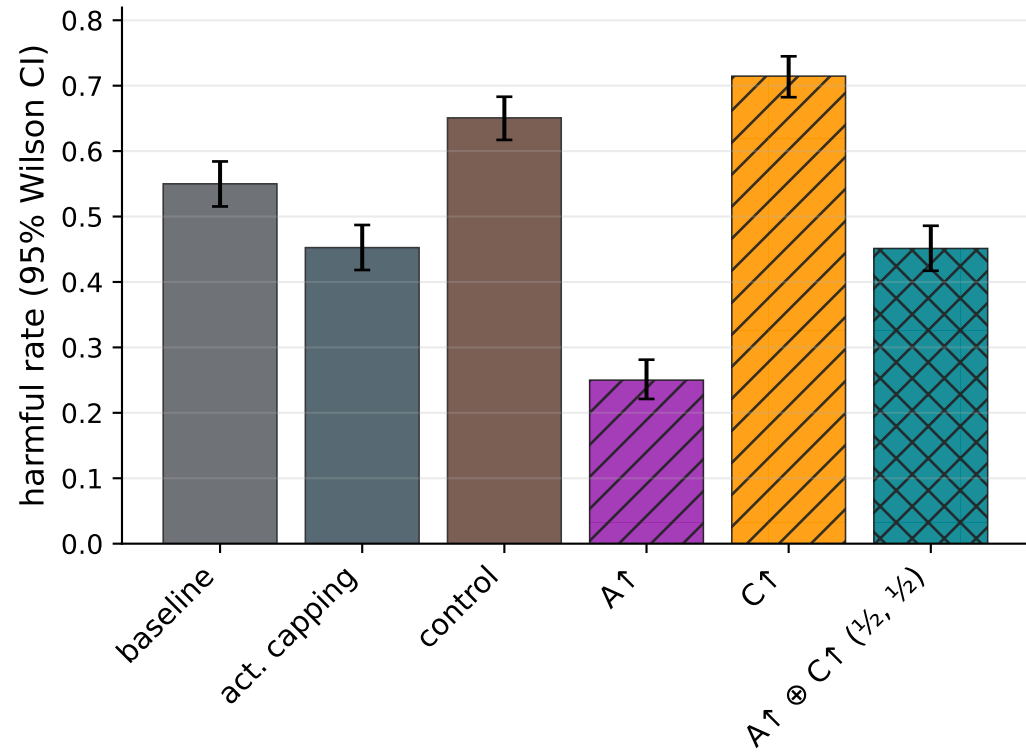
Harmful response rate (WildJailbreak adversarial-harmful)
