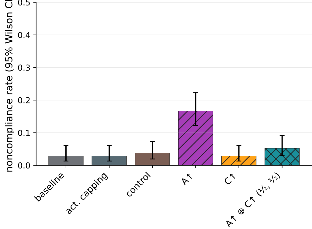
Over-refusal on benign control
