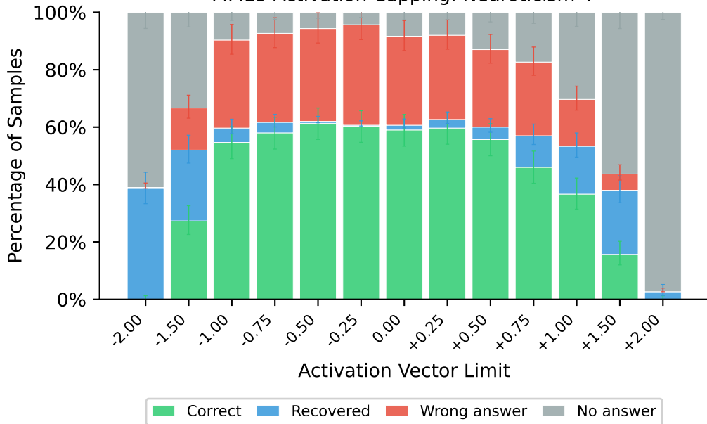
MMLU Activation Capping: Neuroticism ↓
