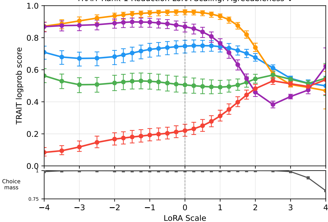
TRAIT Rank-1 Reduction LoRA Scaling: Agreeableness ↓
